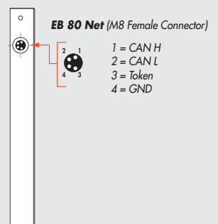
End plate with intermediate control
